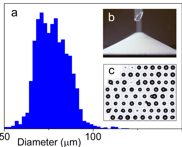
FIG. 2. (Color online) a) Bead size distribution. b) Cone of granular material poured through a funnel, angle of repose \approx 27^\circ , c) Microscopy images of beads (Malvern, Morphology G3) shows the approximate spherical shape of the beads.
