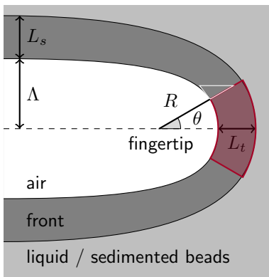
FIG. 10. (Color online) Schematic snapshot of a steadily growing finger. \Lambda is half the finger width, L_s is the front thickness at the sides of the finger, and L_t is the front thickness of the fingertip. The annulus section at the finger tip identifies a small region of the front at the fingertip, bounded by an angle \theta . The maximum curvature of the fingertip is \kappa = 1/R .
