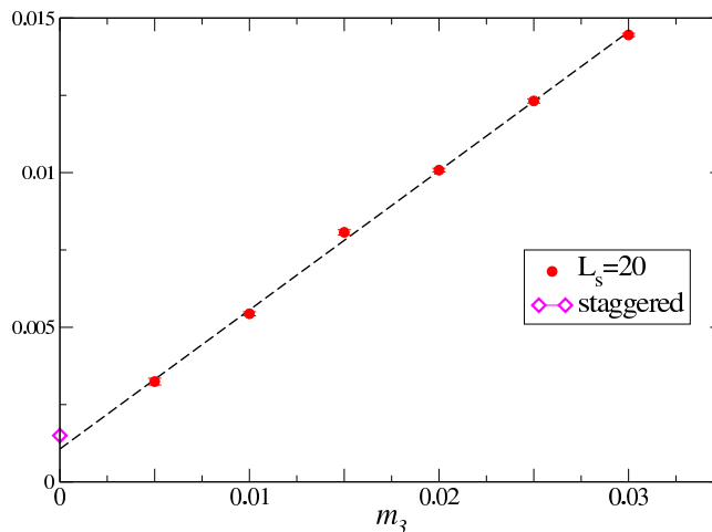
Figure 5. i\langle\bar{\psi}\gamma_3\psi\rangle vs. symmetry-breaking mass m_3 at \beta = 1.0 on 24^3 \times 20 . The diamond shows the corresponding observable extrapolated to the chiral limit using staggered fermions [35].
