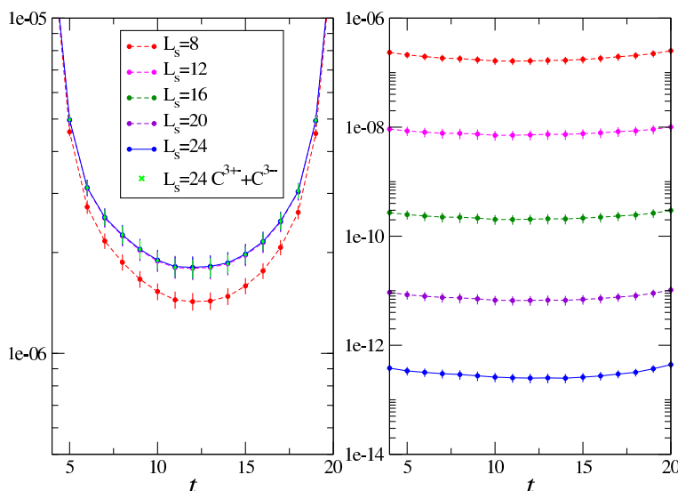
Figure 9. Same as figure 7 but for C^{5+-}(t) (left) and C^{5--}(t) (right). Also shown is the combination C^{3+-}(t) + C^{3--}(t) for L_s = 24 .
