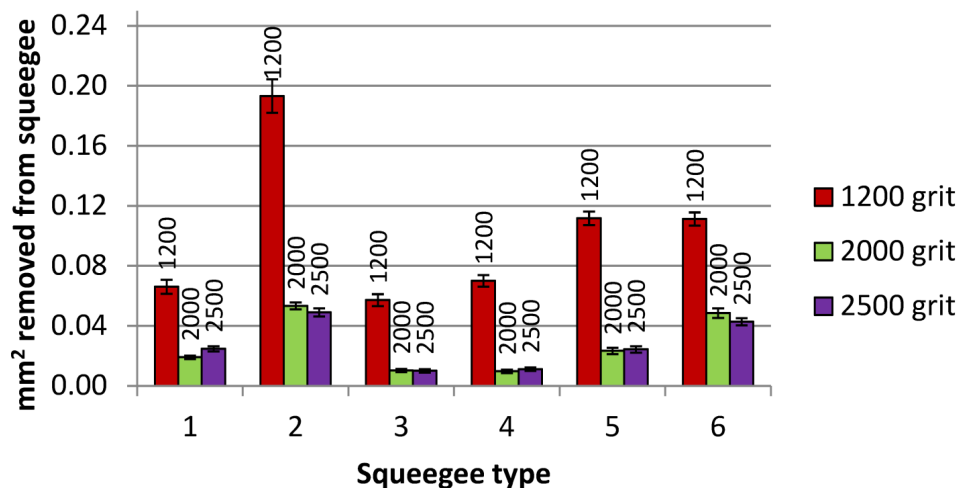
Figure 10. Squeegee cross-sectional area removed after 50 wear cycles with different silicon carbide abrasives. Error bars show standard deviations.
