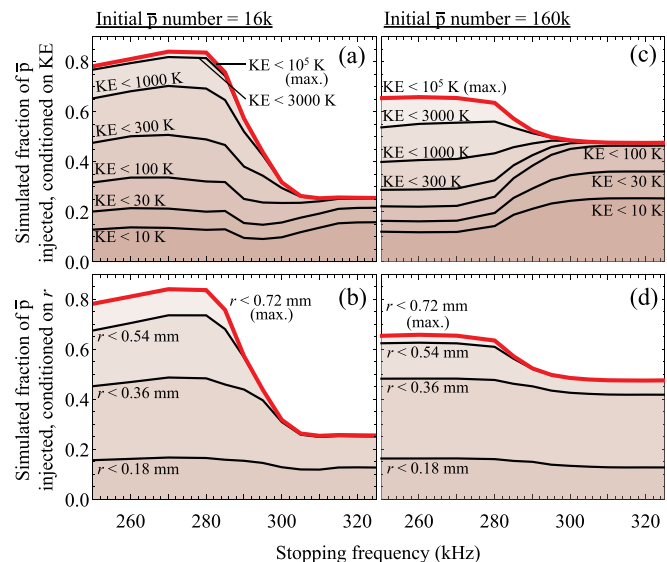
FIG. 9. The simulated, conditional fraction of antiprotons injected into the positron plasma using incremental injection with different stopping frequencies, and two initial antiproton numbers. The rightmost frequency (325 kHz) corresponds to an AR chirp of zero length, with the chirp length increasing towards the left of the horizontal axis. (a) The fraction of antiprotons injected, out of an initial 16000, conditioned on their KE in the positron plasma. (b) Same as a, except that the ratios are conditioned on radius. (c) The fraction of antiprotons injected, out of an initial 160000, conditioned on their KE in the positron plasma. (d) Same as c, except that the ratios are conditioned on radius.
