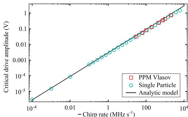
FIG. 3. Critical perturbation amplitude for varying chirp rates. The prediction of the analytic model and the results from the single particle and PPM Vlasov model are compared.
