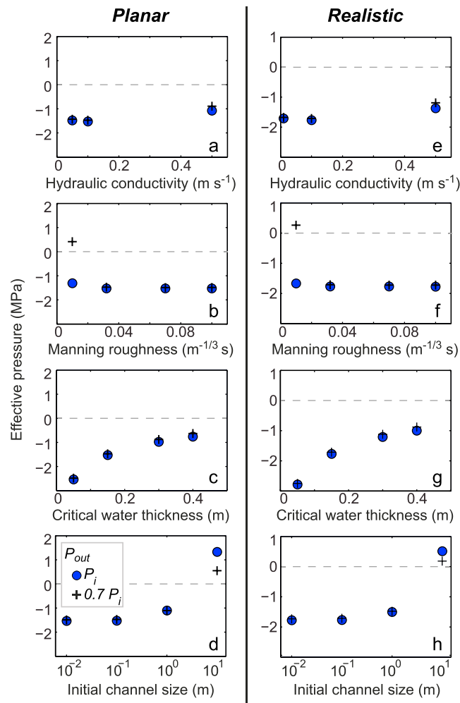
Figure 6. Average effective pressure in the distributed system at 30 days following lake drainage for system outlet water pressures of P_i and 0.7 P_i , plotted as blue circles and black crosses, respectively.
