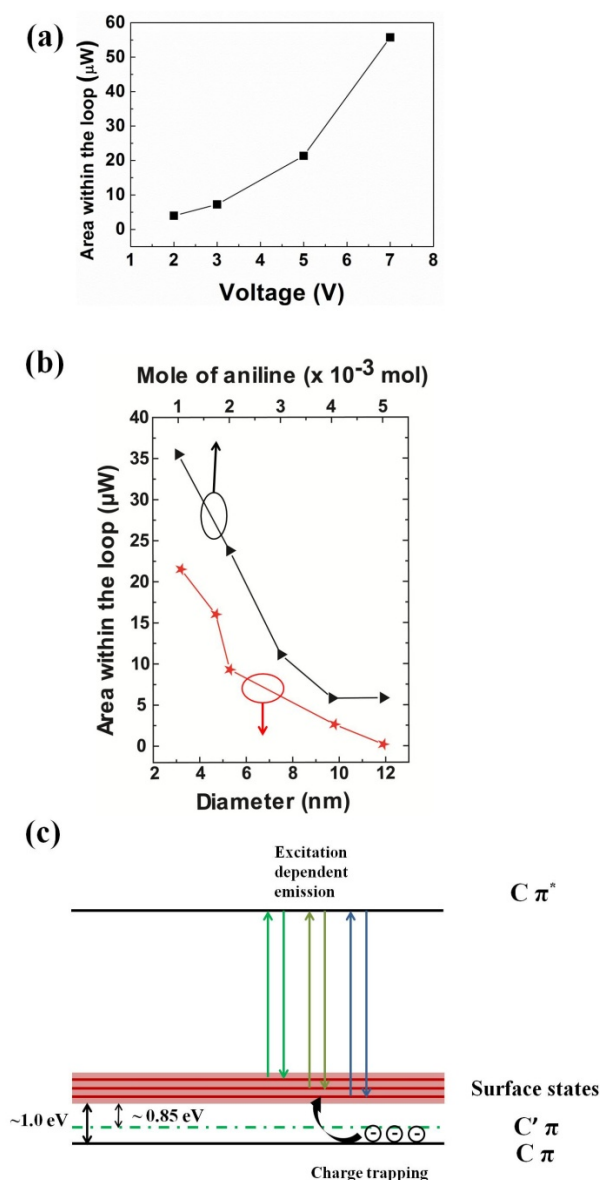
Figure 6 Plot of the area within the hysteresis loops as a function of (a) biased voltage, (b) mole number of aniline and diameter of the GQDs. (c) Schematic diagram of the energy level of the GQDs. The dash line (C'π) indicates the new intrinsic absorption of the PANI-GQD.
