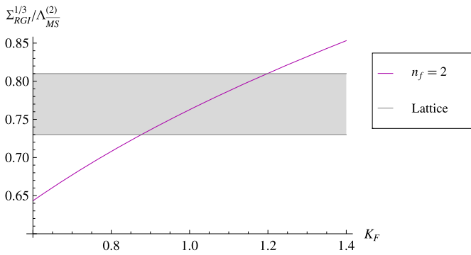
Fig. 5. Plot showing the dependence of the RG-invariant condensate \Sigma_{RG}^{1/3}/\Lambda_{\overline{MS}}^{(n_f)} on the K_F(1/3, n_f) parameter for n_f = 2 superimposed with the one-sigma error band of the lattice determination of Engel et al.
