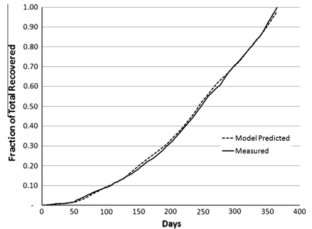
Fig. 8. Comparison of model predicted and measured gold recovery.
