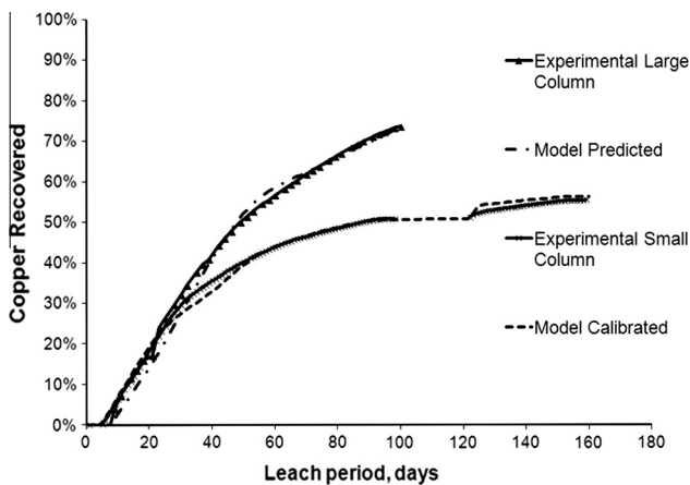
Fig. 3. Copper recovered in pregnant leach solution.
