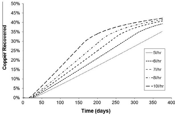
Fig. 9. Copper recovery for various application rates.
