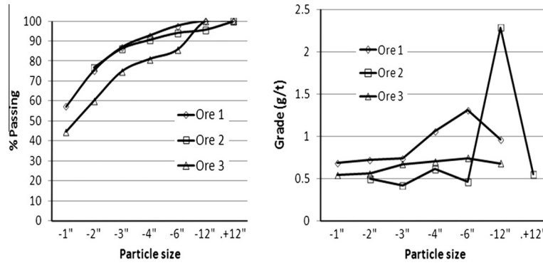
Fig. 5. Particle size distribution and gold grade.
