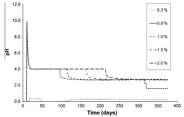
Fig. 13. Acidity of PLS for a range of ore grades.
