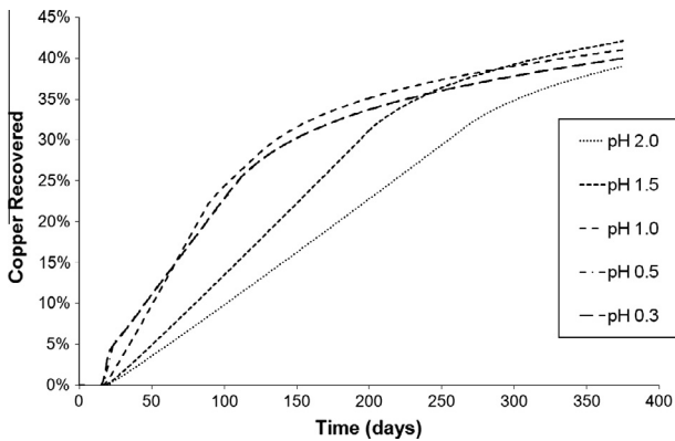
Fig. 11. Copper recovery for different acidity of raffinate.
