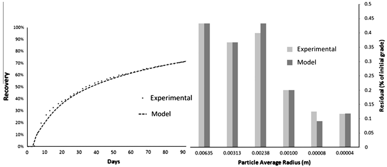
Fig. 2. Calibrated results of copper recovery and copper residual in particle distribution.
