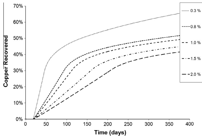
Fig. 14. Copper recovery for a range of ore grades.
