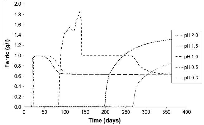
Fig. 12. Ferric in PLS for different acidity of raffinate.
