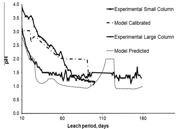
Fig. 4. pH of pregnant leach solution.
