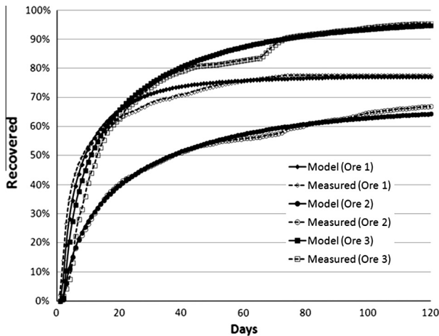
Fig. 6. Percent gold recovered over leach period.
