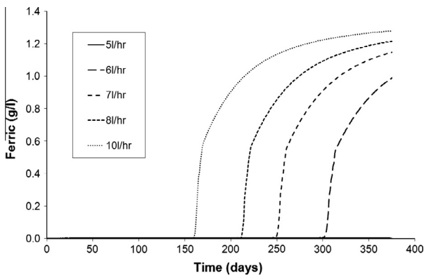
Fig. 10. Ferric in PLS for various application rates.
