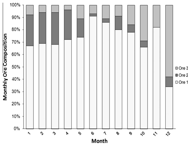
Fig. 7. Composition of material added to heap each month.
