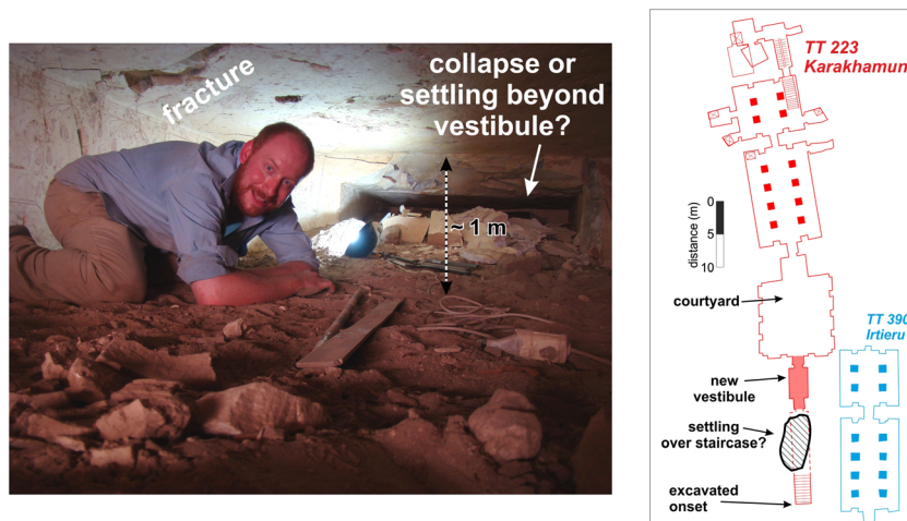
Figure 10. Updated map of the Karakhamun tomb, featuring the new vestibule (solid red in map) that was identified in the 2011 field campaign, and the onset of the descending staircase identified in the following year. The GPR surveys show no evidence of deflected overburden horizons immediately above the vestibule, but develop beyond it (~9 m from the courtyard) at a location consistent with the continuation of the staircase (dashed red lines). This figure is available in colour online at wileyonlinelibrary.com/journal/arp
