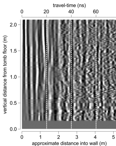
Figure 7. A GPR profile extracted from grid 2, acquired as a vertical CO profile on the internal wall of the Irtieru tomb. No coherent reflections can be identified within this grid that could correspond to the subsurface continuation of the Karakhamun tomb.
