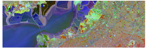
PCA, \gamma = 0.795
