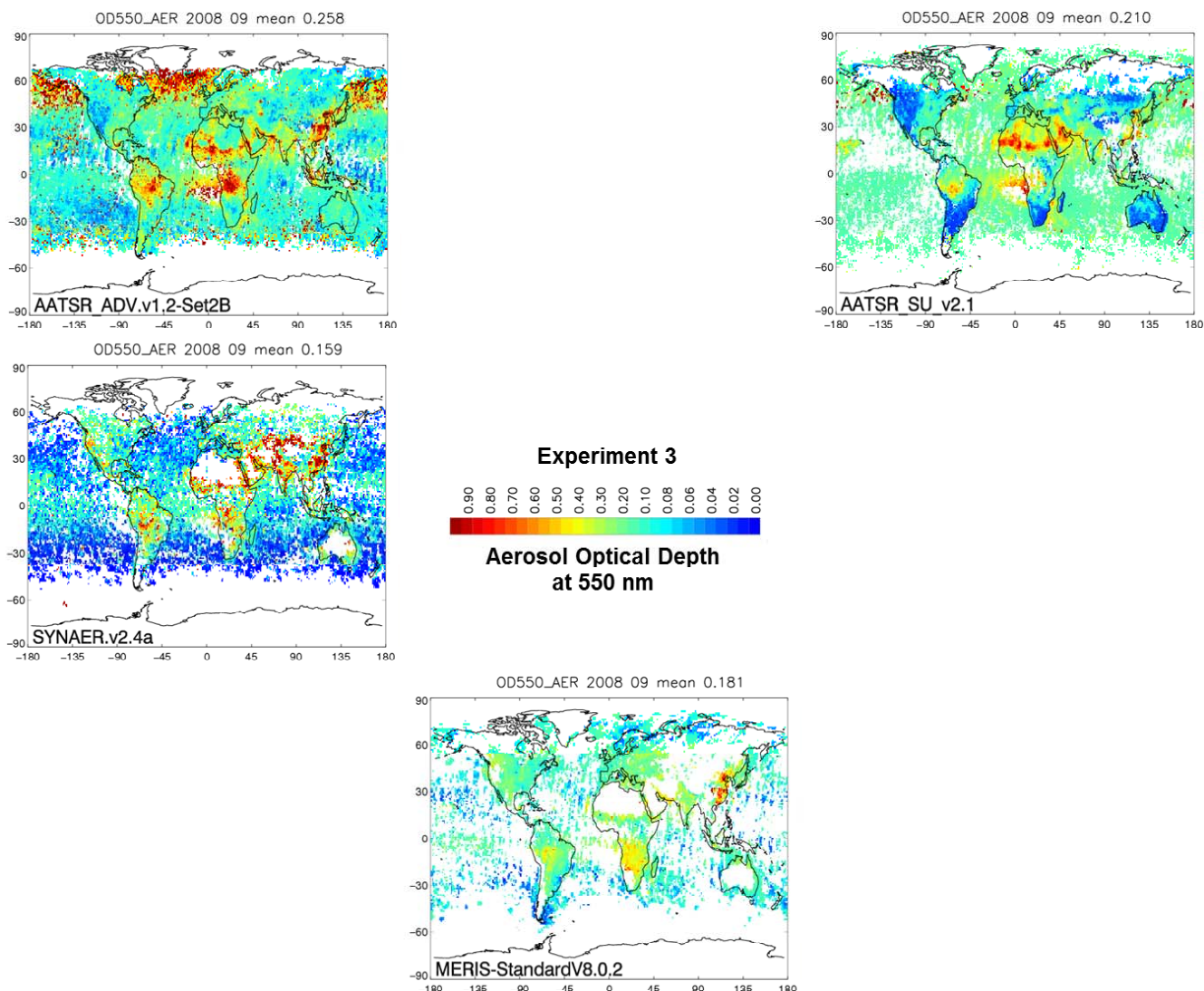
Fig. 9. September 2008 unweighted monthly mean AOD 550 for four total column precursor algorithms as in Fig. 6: datasets with use of common aerosol components and (partly) free retrieval or AeroCom/AERONET climatology as a priori information and common cloud mask (experiment number 3 in Table 1).
