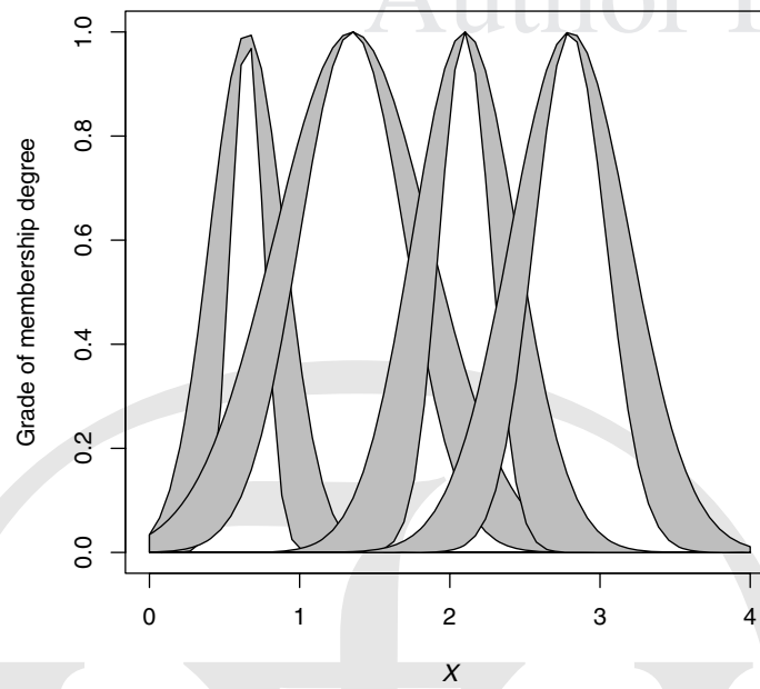
Figure 9. Four aggregated type-2 fuzzy sets.
